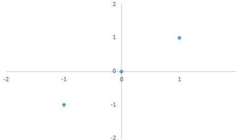
Figure 2: Dataset of the points A(0,0), B(1, 1), C(-1, -1).
